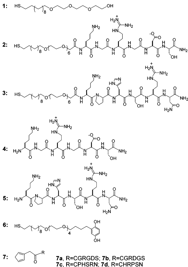
FIGURE 2: Structures of the substituted alkanethiols, hydroquinone conjugate, and peptides used in this work. Compound 1 is the tri(ethylene glycol) terminated alkanethiol. Compounds 2 and 3 are alkanethiols substituted with peptides containing the ligands RGD and PHSRN, respectively. Compounds 4 and 5 are the soluble analogues of the two peptides. Compound 6 is the hydroquinone conjugate used on SAMs to immobilize cyclopentadiene-peptide conjugates 7 .
